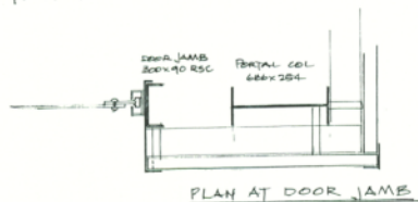
PLAN AT DOOR JAMB
