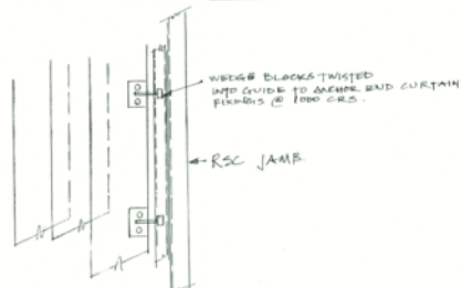
ELEVATION AT DOOR JAMB
