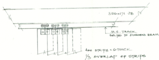
ELEVATION AT HEAD
